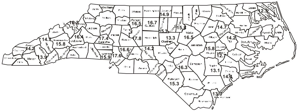
Figure 5.6 PM 2.5 : Maximum Annual Arithmetic Means, 2000
