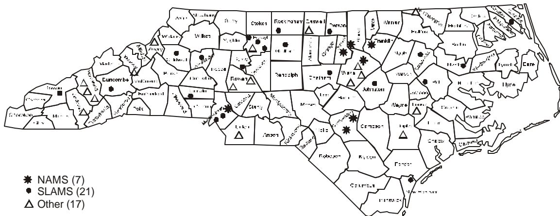
Figure 5.10 Location of Ozone Monitoring Sites
