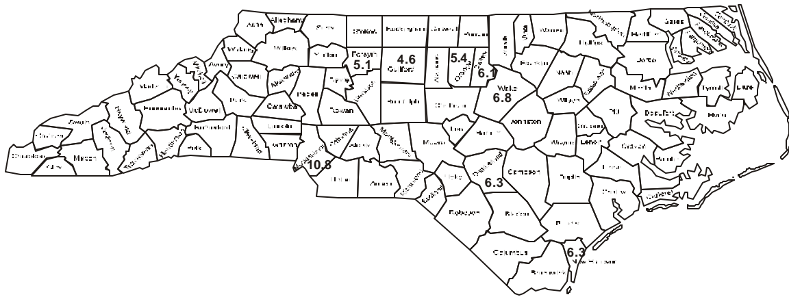
Figure 5.8 Carbon Monoxide: Second Highest 1-Hour Average, 2000
