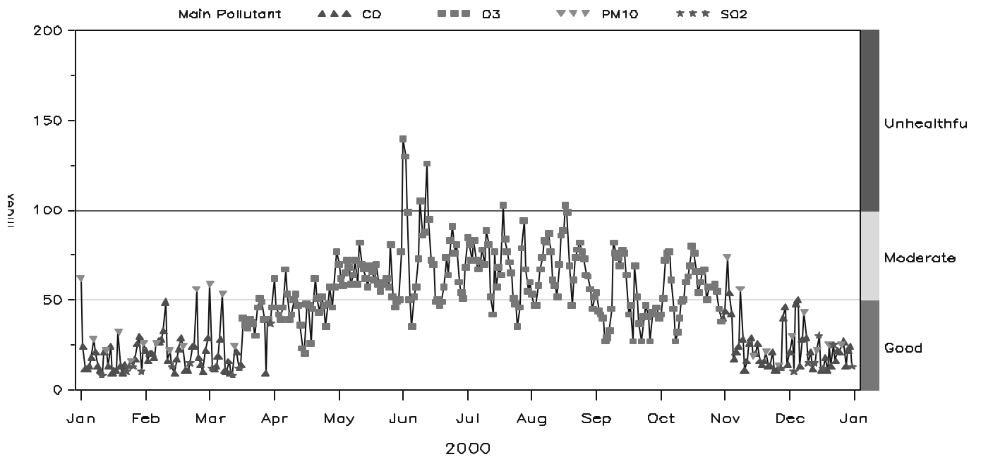
Figure 6.2 Daily Air Quality Values for Charlotte-Gastonia, NC,-Rock Hill, SC, Metropolitan Statistical Area, 2000
