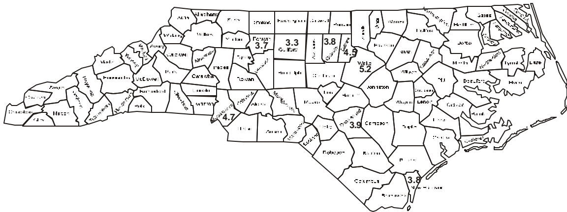
Figure 5.9 Carbon Monoxide: Second Highest Non-overlapping 8-Hour Average, 2000
