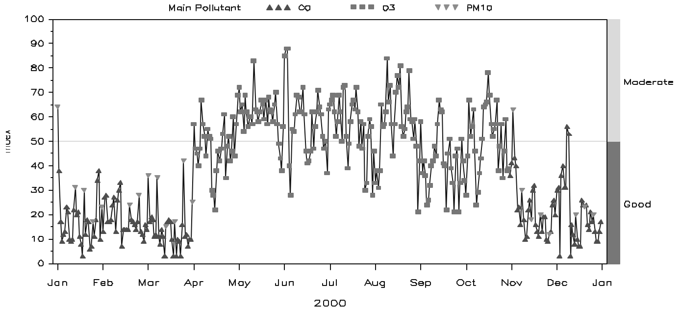
Figure 6.3 Daily Air Quality Index Values for Fayetteville, NC, Metropolitan Statistical Area, 2000
