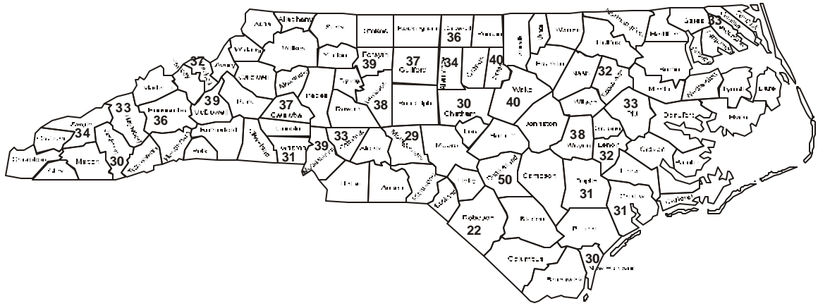
Figure 5.5 PM 2.5 : Second Highest 24-Hour Averages, 2000
