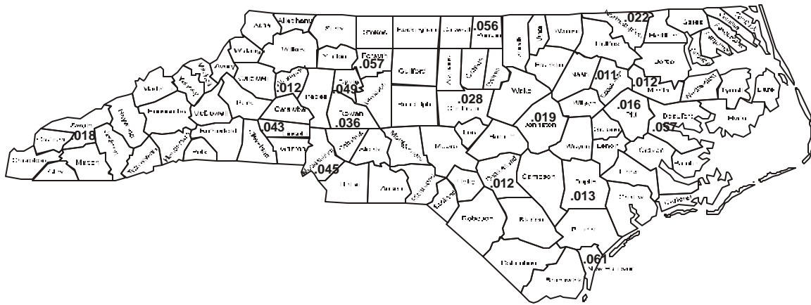
Figure 5.17 Sulfur Dioxide: Second Highest 3-Hour Averages in the Most Recent Year of Data from 1998, 1999 or 2000
