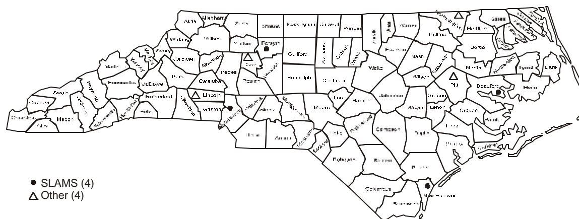
Figure 5.16 Location of Sulfur Dioxide Monitoring Sites
