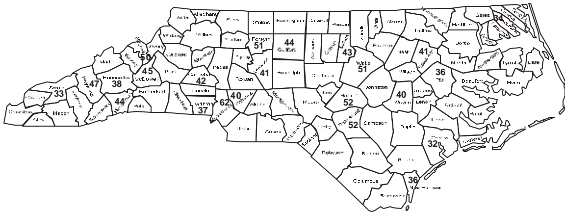
Figure 5.2 PM 10 : Second Highest 24-Hour Averages, 2000
