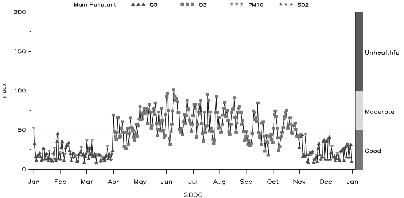
Figure 6.4 Daily Air Quality Index Values Greensboro-Winston-Salem-High Point, NC, Metropolitan Statistical Area, 2000
