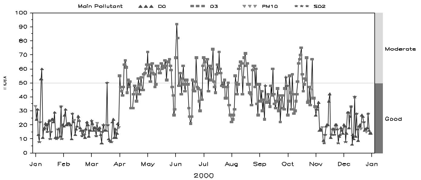
Figure 6.6 Daily Air Quality Index Values for Wilmington, NC, Metropolitan Statistical Area, 2000
