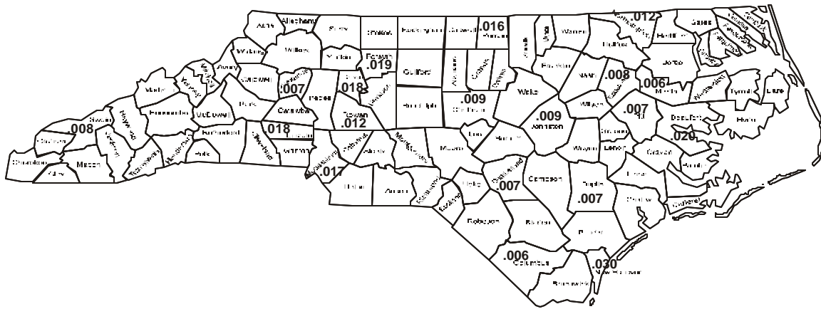
Figure 5.18 Sulfur Dioxide: Second Highest 24-Hour Averages in the Most Recent Year of Data from 1998, 1999 or 2000
