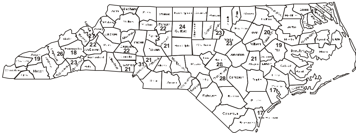
Figure 5.3 PM 10 : Maximum Annual Arithmetic Means, 2000
