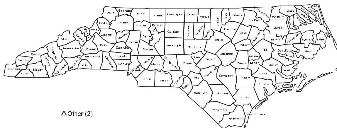
Figure 5.19 Location of Nitrogen Dioxide Monitoring Sites
