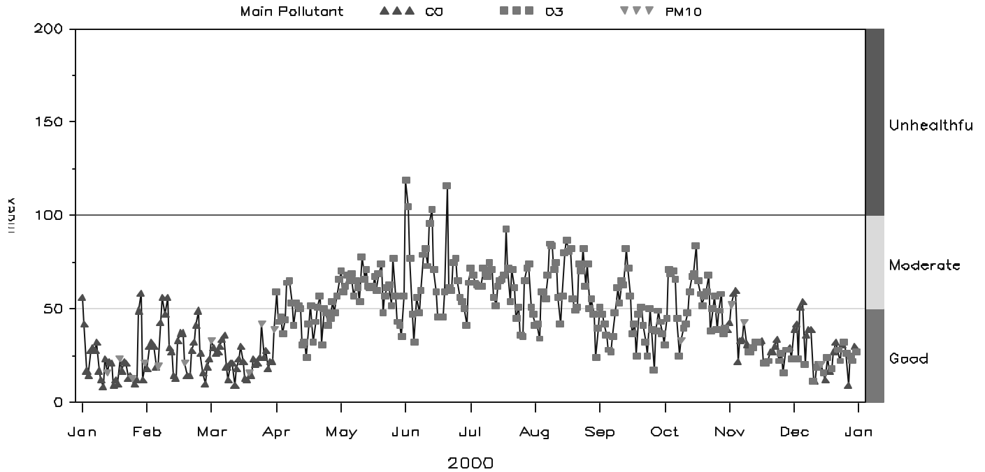
Figure 6.5 Daily Air Quality Index Values for Raleigh-Durham, NC, Metropolitan Statistical Area, 2000
