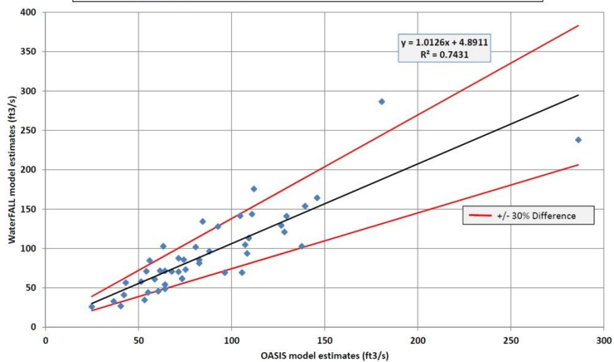
OASIS & WaterFALL Comparison - Buffalo Creek, DWR IFIM Site (127 mi 2 ) November Monthly Medians (1961-2006, calendar year)
