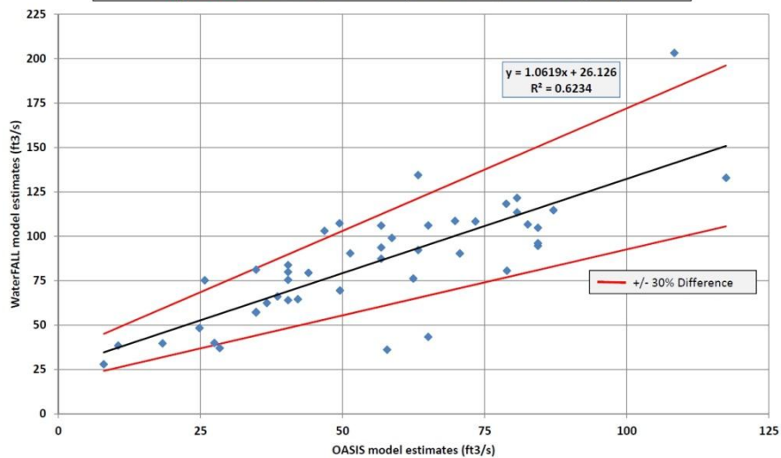
OASIS & WaterFALL Comparison - Buffalo Creek, DWR IFIM Site (127 mi 2 ) September Monthly Medians (1961-2006, calendar year)
