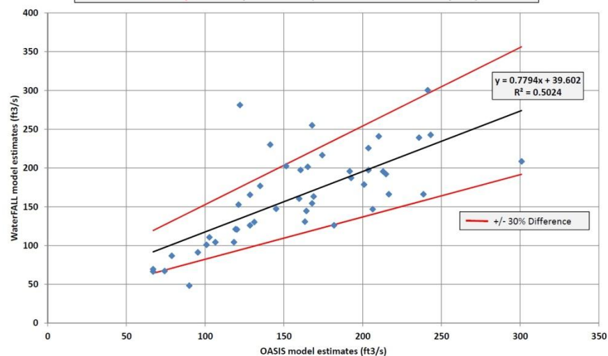
OASIS & WaterFALL Comparison - Buffalo Creek, DWR IFIM Site (127 mi 2 ) February Monthly Medians (1961-2006, calendar year)
