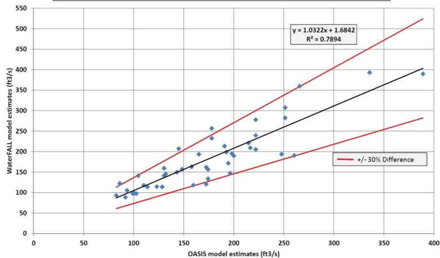
OASIS & WaterFALL Comparison - Buffalo Creek, DWR IFIM Site (127 mi 2 ) March Monthly Medians (1961-2006, calendar year)
