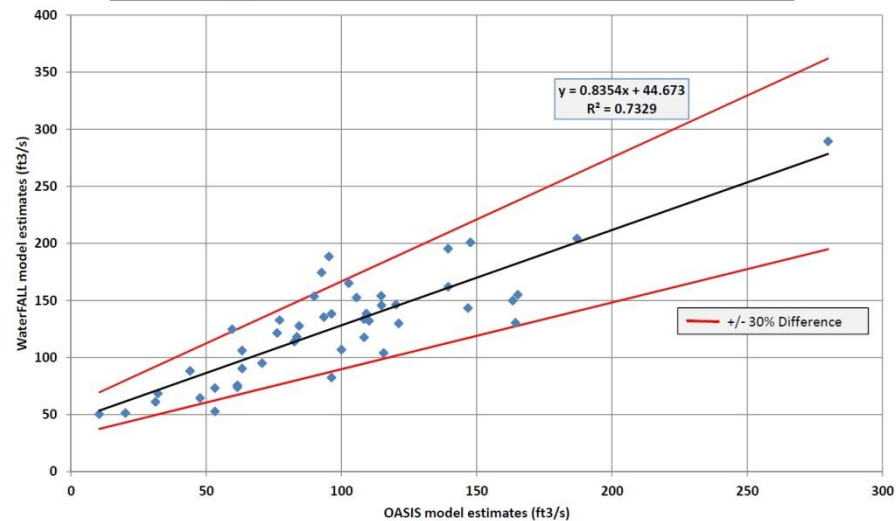
OASIS & WaterFALL Comparison - Buffalo Creek, DWR IFIM Site (127 mi 2 ) June Monthly Medians (1961-2006, calendar year)
