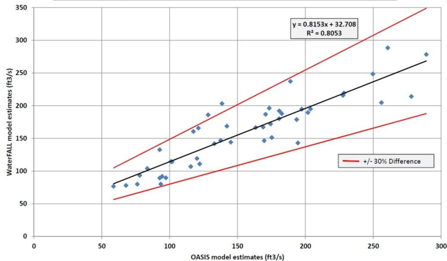
OASIS & WaterFALL Comparison - Buffalo Creek, DWR IFIM Site (127 mi 2 ) April Monthly Medians (1961-2006, calendar year)
