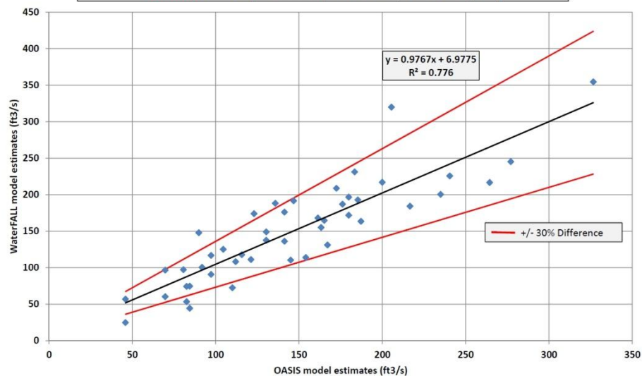
OASIS & WaterFALL Comparison - Buffalo Creek, DWR IFIM Site (127 mi 2 ) January Monthly Medians (1961-2006, calendar year)
