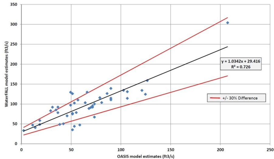
OASIS & WaterFALL Comparison - Buffalo Creek, DWR IFIM Site (127 mi 2 ) August Monthly Medians (1961-2006, calendar year)
