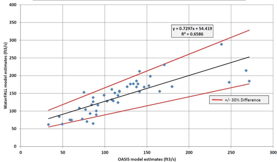
OASIS & WaterFALL Comparison - Buffalo Creek, DWR IFIM Site (127 mi 2 ) May Monthly Medians (1961-2006, calendar year)
