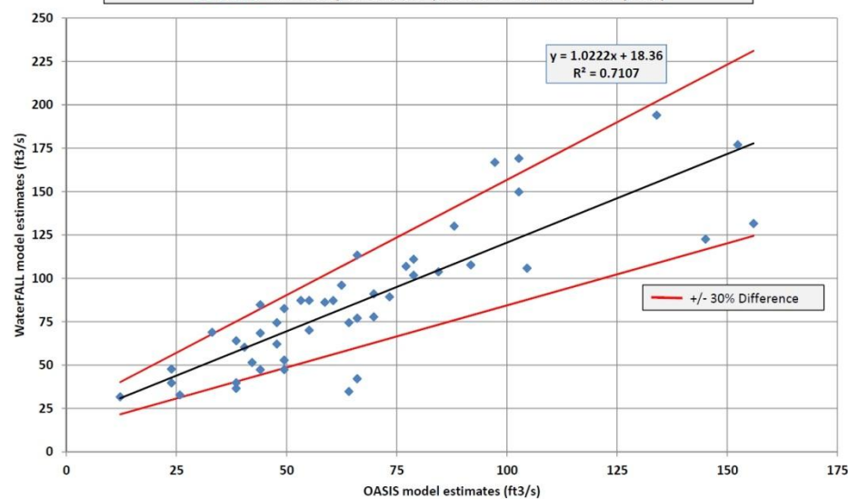
OASIS & WaterFALL Comparison - Buffalo Creek, DWR IFIM Site (127 mi 2 ) October Monthly Medians (1961-2006, calendar year)
