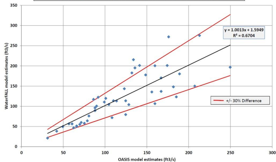
OASIS & WaterFALL Comparison - Buffalo Creek, DWR IFIM Site (127 mi 2 ) December Monthly Medians (1961-2006, calendar year)
