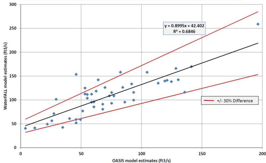
OASIS & WaterFALL Comparison - Buffalo Creek, DWR IFIM Site (127 mi 2 ) July Monthly Medians (1961-2006, calendar year)
