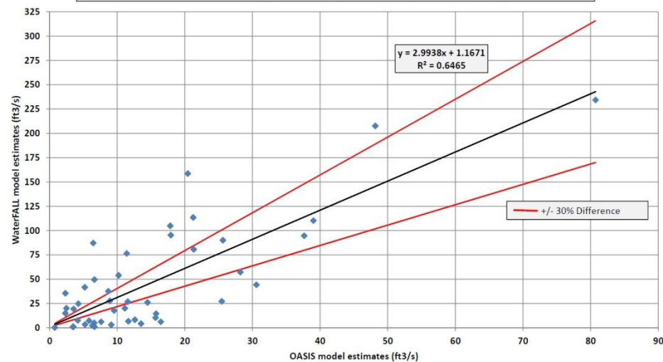
OASIS & WaterFALL Comparison - Eno River, State Park DWR IFIM Site (99.4 mi 2 ) October Monthly Medians (1961-2006, calendar year)
