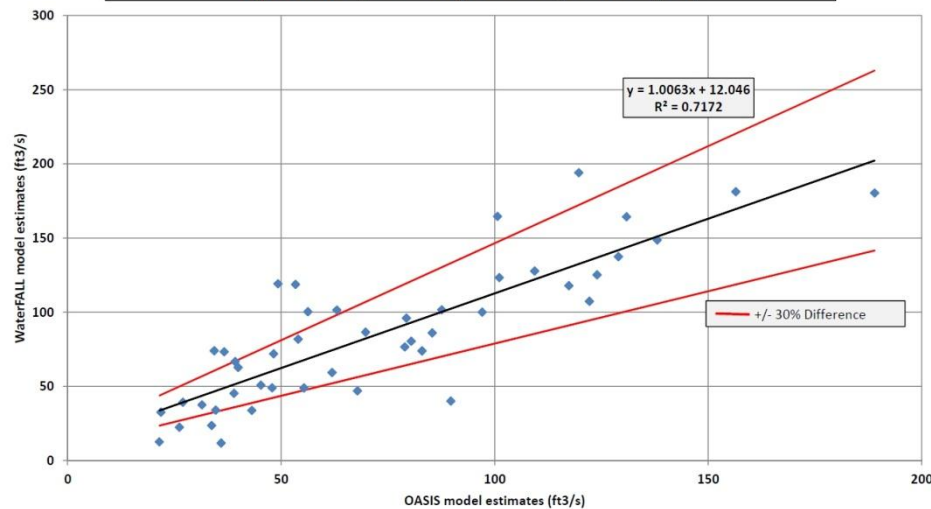
OASIS & WaterFALL Comparison - Eno River, State Park DWR IFIM Site (99.4 mi 2 ) April Monthly Medians (1961-2006, calendar year)
