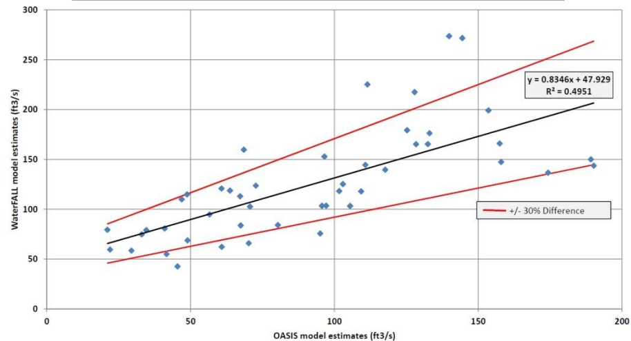
OASIS & WaterFALL Comparison - Eno River, State Park DWR IFIM Site (99.4 mi 2 ) February Monthly Medians (1961-2006, calendar year)
