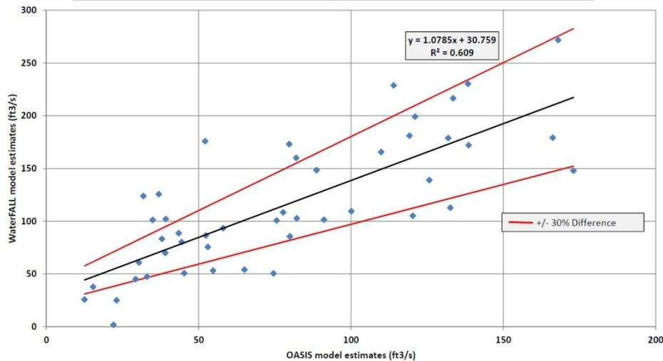
OASIS & WaterFALL Comparison - Eno River, State Park DWR IFIM Site (99.4 mi 2 ) January Monthly Medians (1961-2006, calendar year)
