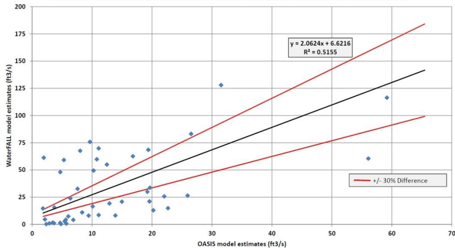
OASIS & WaterFALL Comparison - Eno River, State Park DWR IFIM Site (99.4 mi 2 ) September Monthly Medians (1961-2006, calendar year)
