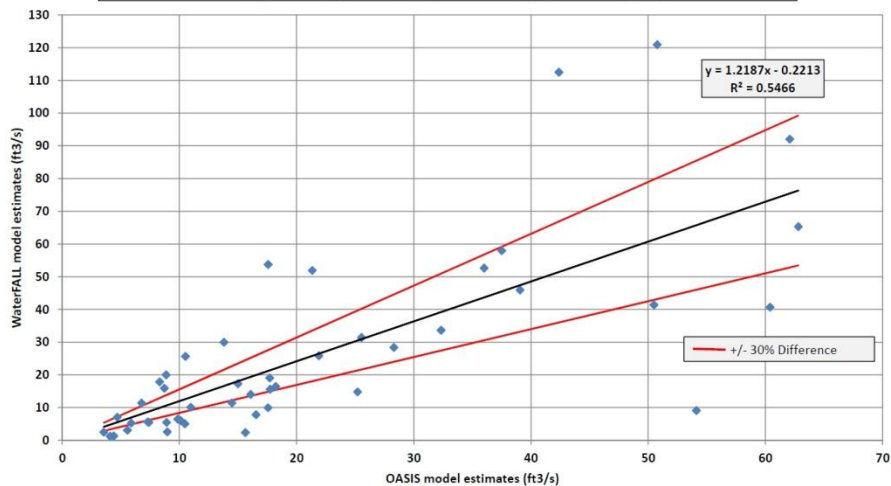
OASIS & WaterFALL Comparison - Eno River, State Park DWR IFIM Site (99.4 mi 2 ) July Monthly Medians (1961-2006, calendar year)
