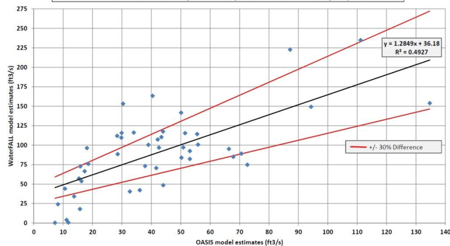
OASIS & WaterFALL Comparison - Eno River, State Park DWR IFIM Site (99.4 mi 2 ) December Monthly Medians (1961-2006, calendar year)
