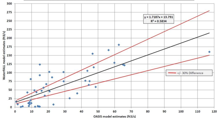
OASIS & WaterFALL Comparison - Eno River, State Park DWR IFIM Site (99.4 mi 2 ) November Monthly Medians (1961-2006, calendar year)
