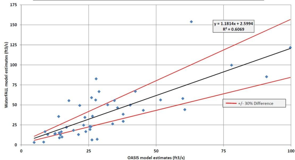
OASIS & WaterFALL Comparison - Eno River, State Park DWR IFIM Site (99.4 mi 2 ) June Monthly Medians (1961-2006, calendar year)
