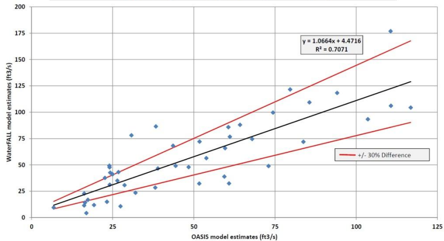
OASIS & WaterFALL Comparison - Eno River, State Park DWR IFIM Site (99.4 mi 2 ) May Monthly Medians (1961-2006, calendar year)
