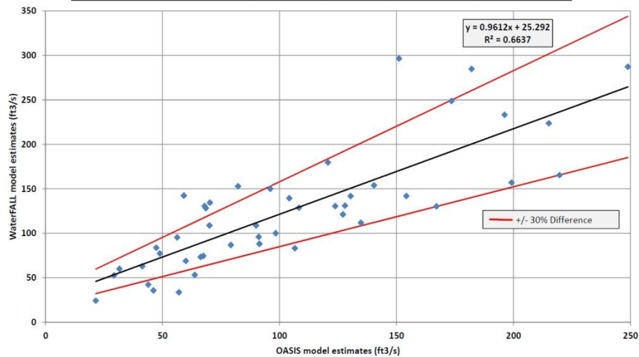
OASIS & WaterFALL Comparison - Eno River, State Park DWR IFIM Site (99.4 mi 2 ) March Monthly Medians (1961-2006, calendar year)
