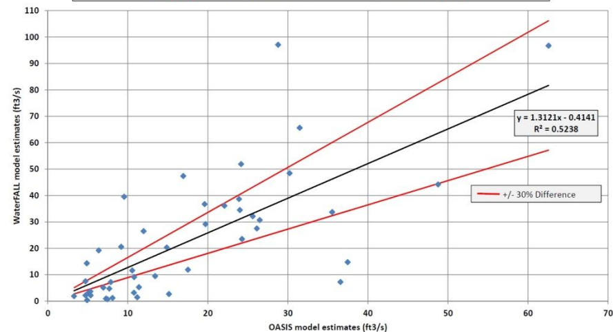
OASIS & WaterFALL Comparison - Eno River, State Park DWR IFIM Site (99.4 mi 2 ) August Monthly Medians (1961-2006, calendar year)
