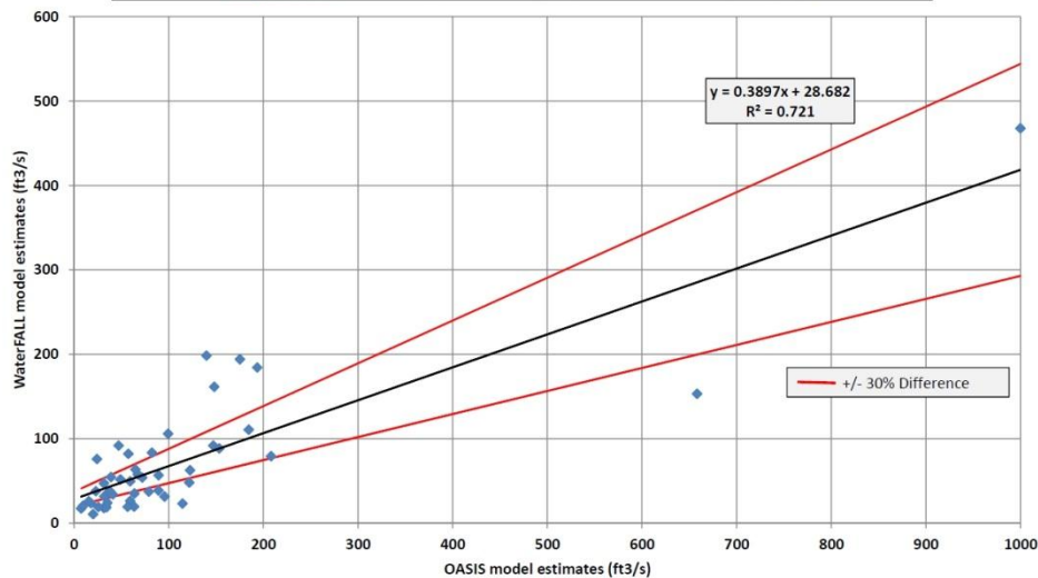
OASIS & WaterFALL Comparison - Tar River, Louisburg DWR IFIM Site (437 mi 2 ) September Monthly Medians (1961-2006, calendar year)
