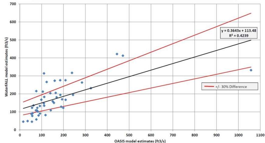
OASIS & WaterFALL Comparison - Tar River, Louisburg DWR IFIM Site (437 mi 2 ) June Monthly Medians (1961-2006, calendar year)
