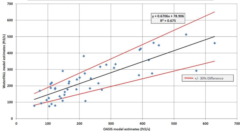
OASIS & WaterFALL Comparison - Tar River, Louisburg DWR IFIM Site (437 mi 2 ) May Monthly Medians (1961-2006, calendar year)
