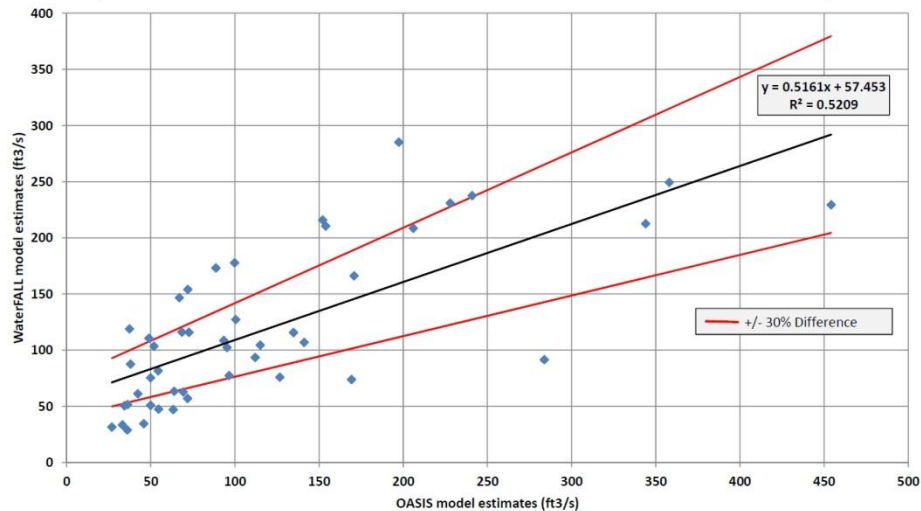
OASIS & WaterFALL Comparison - Tar River, Louisburg DWR IFIM Site (437 mi 2 ) July Monthly Medians (1961-2006, calendar year)
