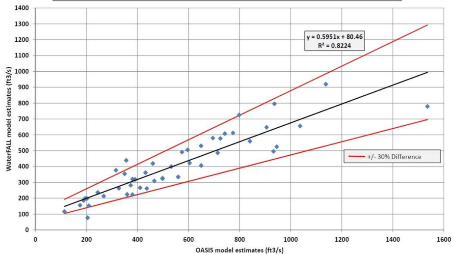
OASIS & WaterFALL Comparison - Tar River, Louisburg DWR IFIM Site (437 mi 2 ) March Monthly Medians (1961-2006, calendar year)
