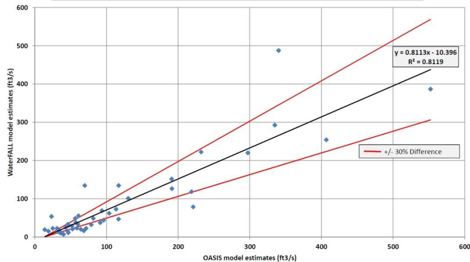
OASIS & WaterFALL Comparison - Tar River, Louisburg DWR IFIM Site (437 mi 2 ) October Monthly Medians (1961-2006, calendar year)
