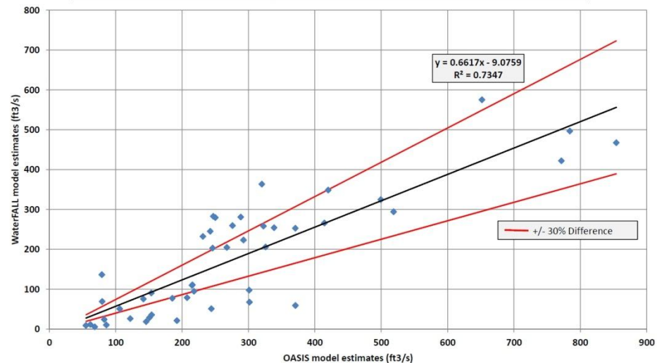
OASIS & WaterFALL Comparison - Tar River, Louisburg DWR IFIM Site (437 mi 2 ) December Monthly Medians (1961-2006, calendar year)
