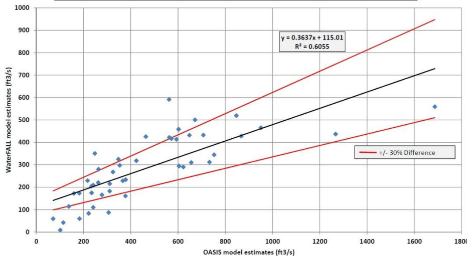
OASIS & WaterFALL Comparison - Tar River, Louisburg DWR IFIM Site (437 mi 2 ) January Monthly Medians (1961-2006, calendar year)
