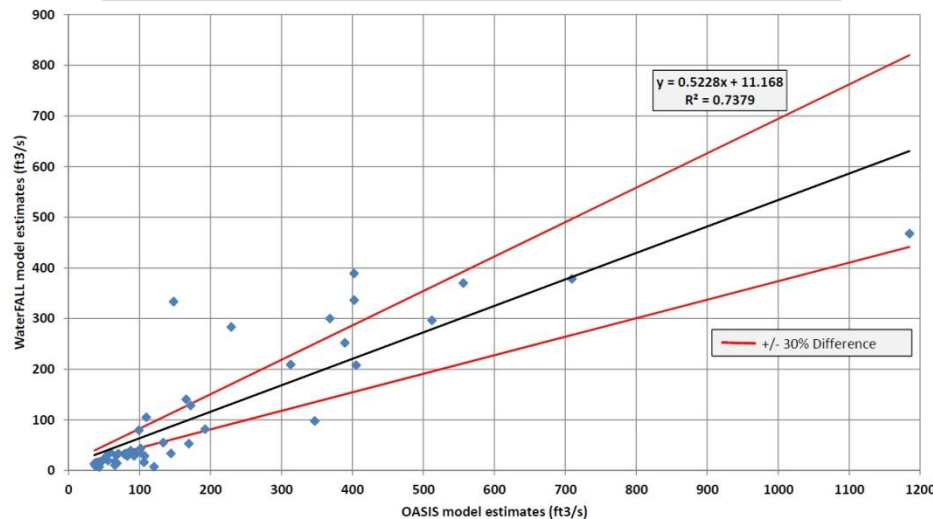
OASIS & WaterFALL Comparison - Tar River, Louisburg DWR IFIM Site (437 mi 2 ) November Monthly Medians (1961-2006, calendar year)
