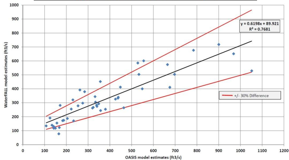
OASIS & WaterFALL Comparison - Tar River, Louisburg DWR IFIM Site (437 mi 2 ) April Monthly Medians (1961-2006, calendar year)
