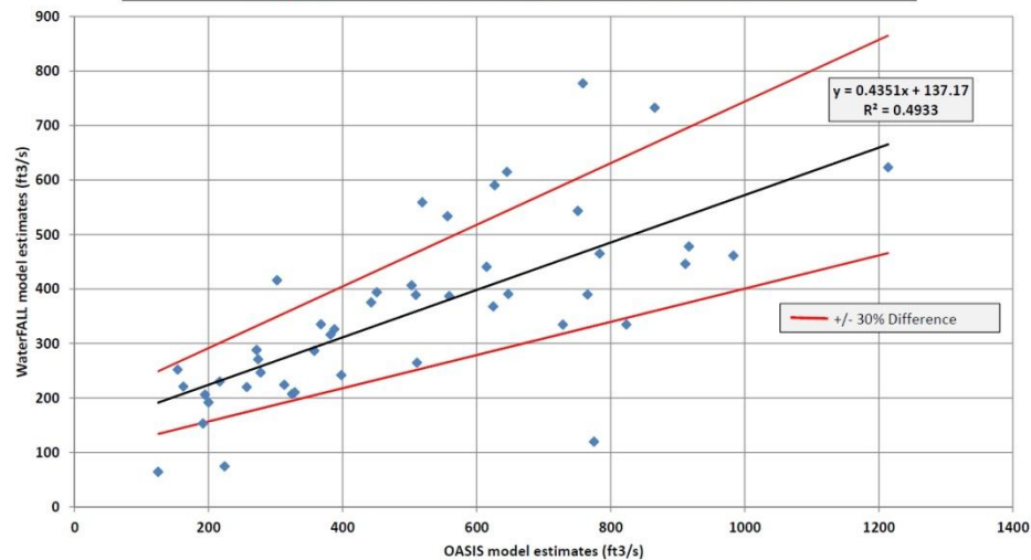
OASIS & WaterFALL Comparison - Tar River, Louisburg DWR IFIM Site (437 mi 2 ) February Monthly Medians (1961-2006, calendar year)
