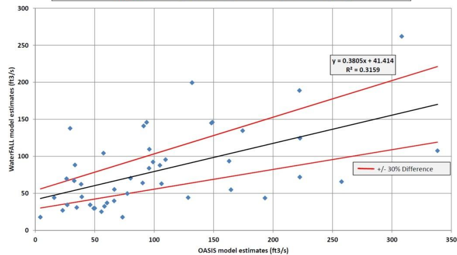
OASIS & WaterFALL Comparison - Tar River, Louisburg DWR IFIM Site (437 mi 2 ) August Monthly Medians (1961-2006, calendar year)
