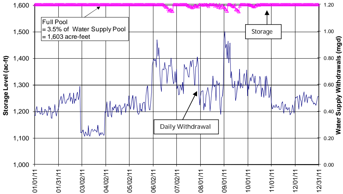
Figure 4. RTP South Water Supply Allocation and Withdrawals for 2011
