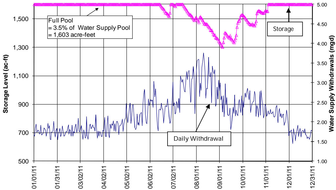
Figure 3. Morrisville Water Supply Allocation and Withdrawals for 2011
