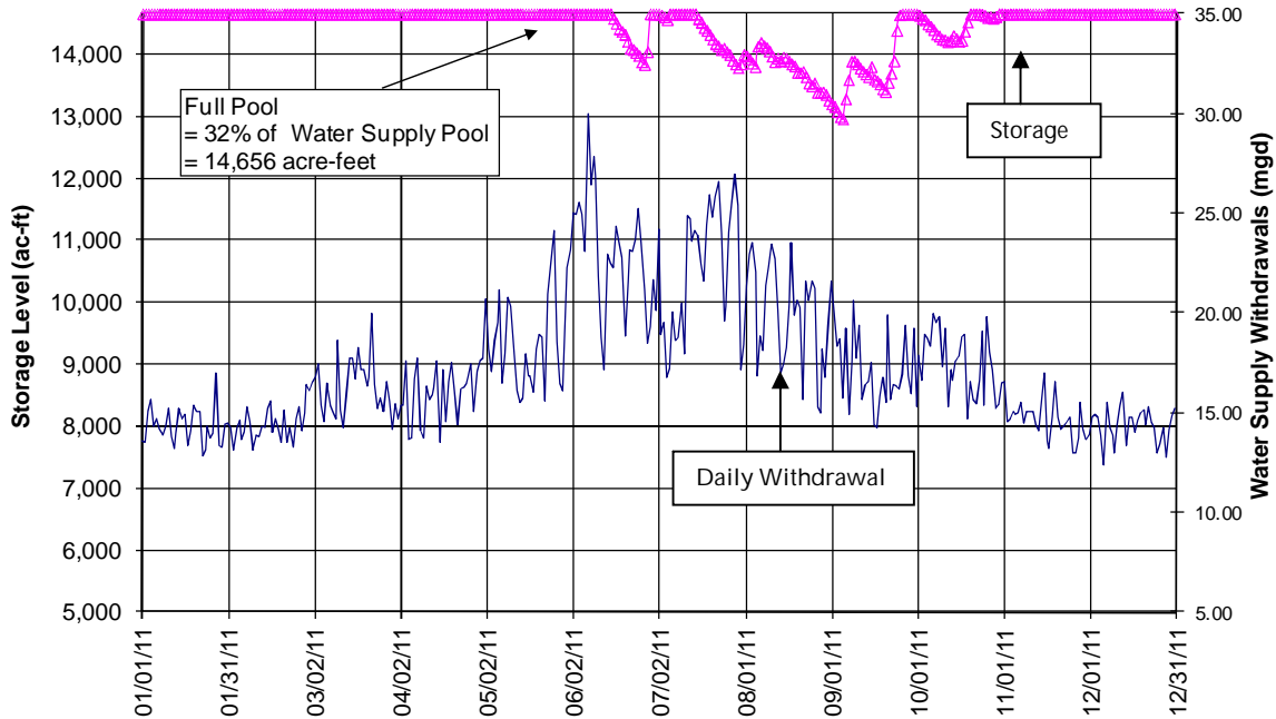
Figure 2. Cary/Apex Water Supply Allocation and Withdrawals for 2011
